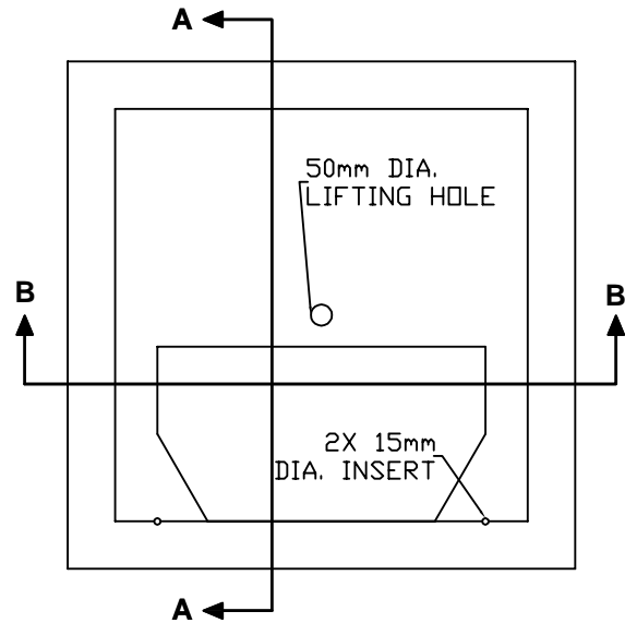
PAD (PLAN VIEW)
