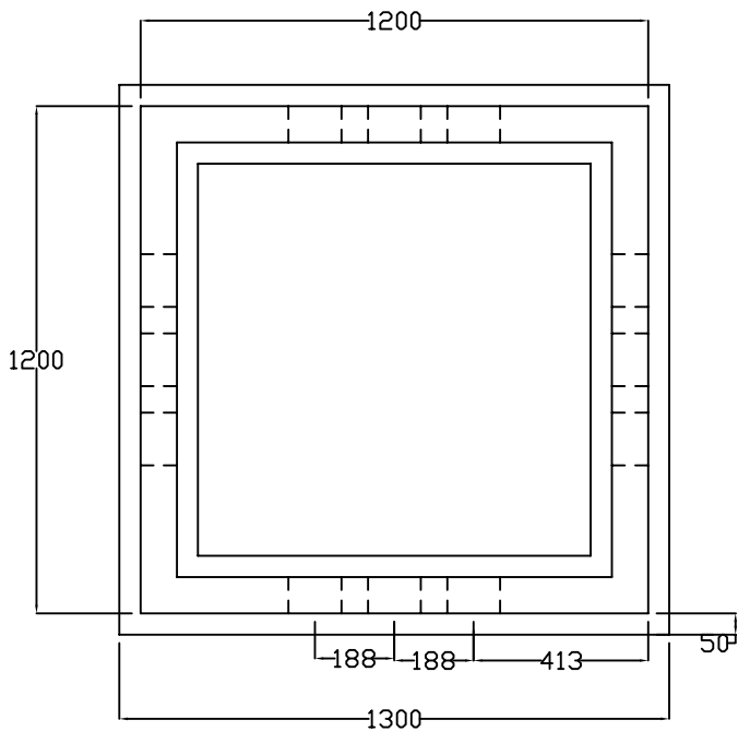
BASE (PLAN VIEW)
